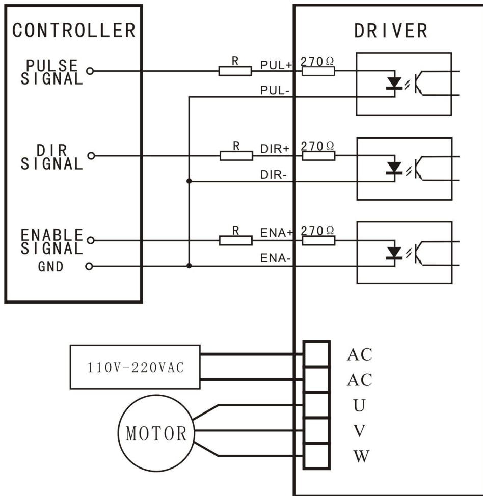
Figure 3: Typical connection
